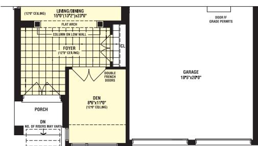
PARTIAL GROUND FLOOR PLAN 'S'
