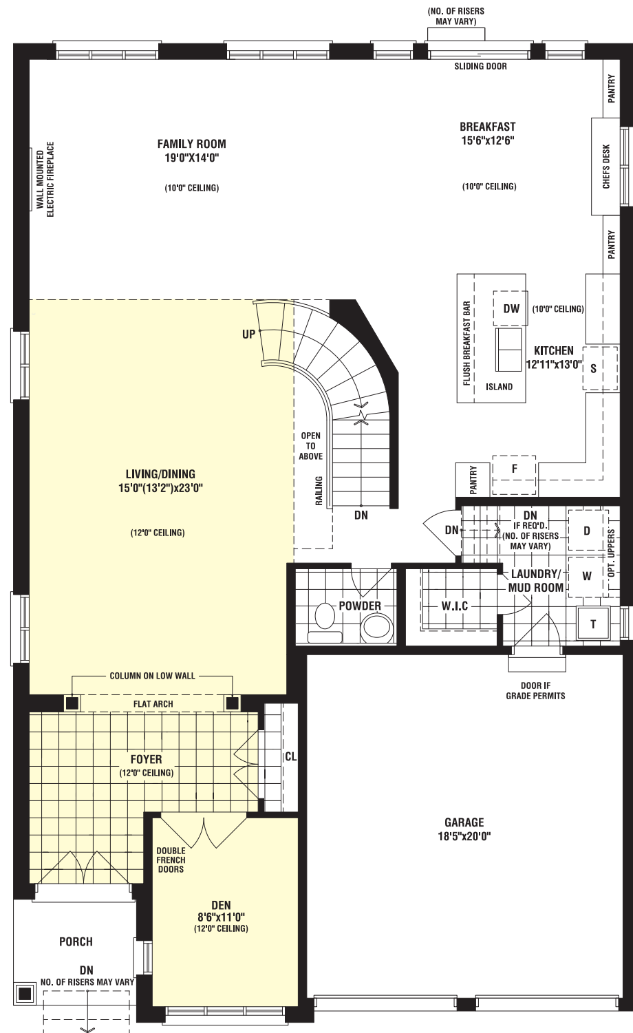
GROUND FLOOR PLAN ELEV. 'A'
