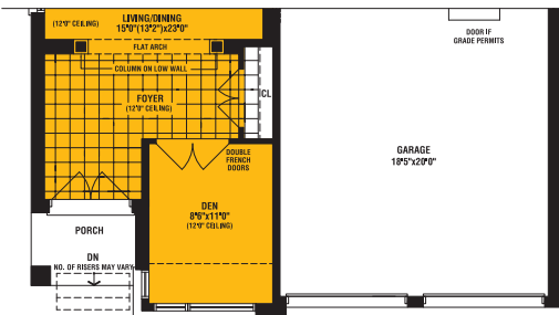
PARTIAL GROUND FLOOR PLAN 'M'
