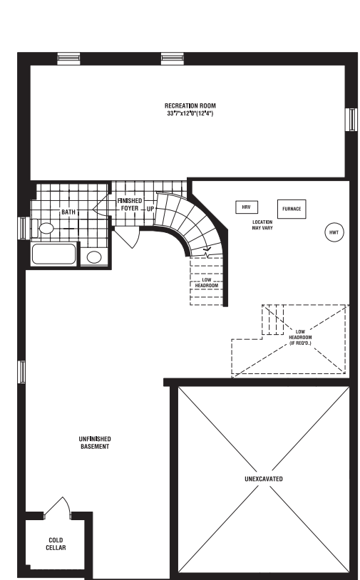
BASEMENT PLAN ELEV. 'M'
