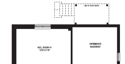
PARTIAL BASEMENT PLAN 'A' & 'B' W.D.O. CONDITION
