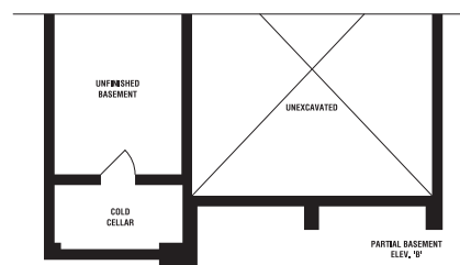
PARTIAL BASEMENT ELEV. 'B'
