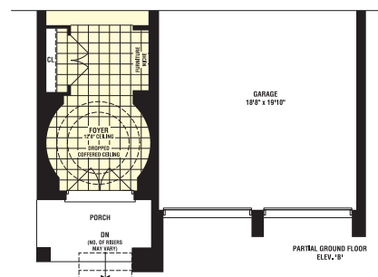
PARTIAL GROUND FLOOR PLAN 'A' & 'B' W.O.B. CONDITION
